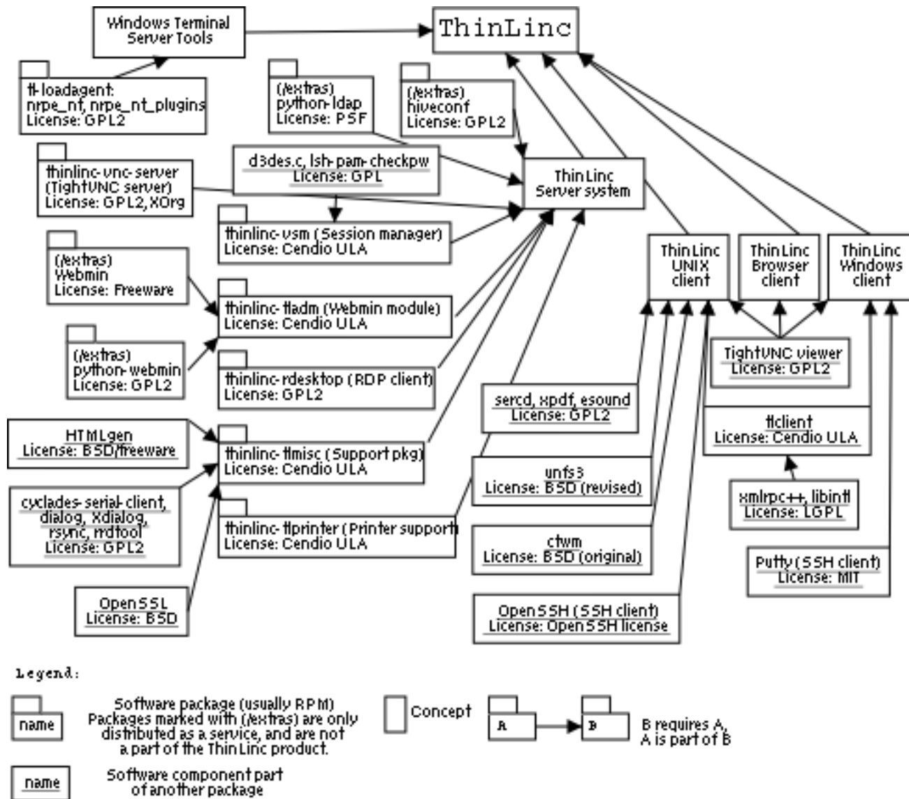
Figure 1-1. ThinLinc Components
